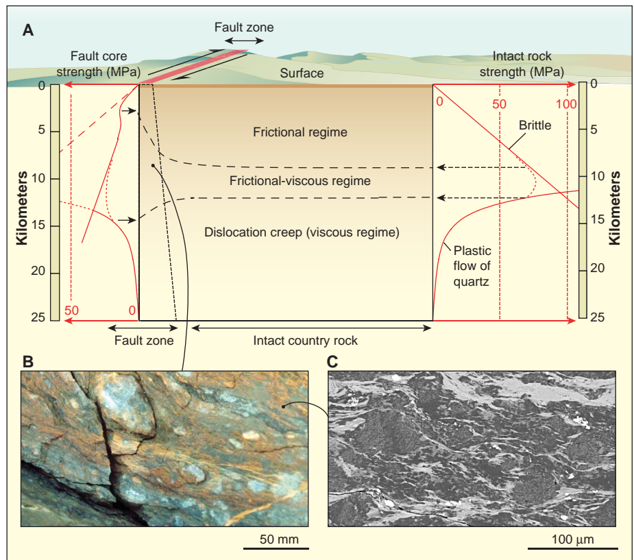
The microphysics of faults. (A) Right side, experimentally derived strength-versus-depth profiles for intact rock (5) based on traditional brittle-plastic rheology. Left side, strength profile for a vertical fault, with a broadened mid-crustal “frictional-viscous” regime characteristic of a weak, fluid-infiltrated and altered fault zone (9). (B) Natural example of brittle cataclasite breccia overprinted by mica-rich foliation, representing a transition to frictional-viscous behavior. (C) Scanning electron microscope image of foliated fault rock in which the mica-rich layers formed by alteration of feldspars form an interconnected weak layer at the microscopic scale. Images in bottom panel are of fault rocks from core of Median Tectonic Line, Japan (taken by S. Jefferies and M. Albers).
