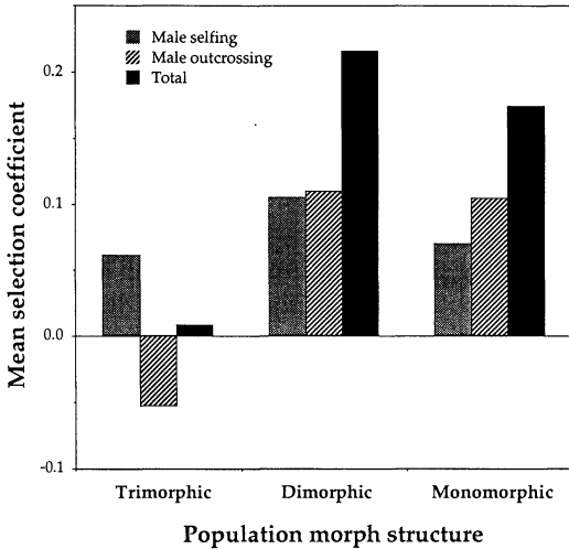
FIG. 2. Mean selection coefficient [ I = 1 - (W'_M)/W_M ] favoring the M' over the M morphology under different morph structures in experimental populations of Eichhornia paniculata . The total selection coefficient was decomposed into male selfing [ (S_M' - S_M)/W_M ] and male outcrossing [ (P_M' - P_M)/W_M ] sources to illustrate the strength and direction of selection on different components of reproductive success.
