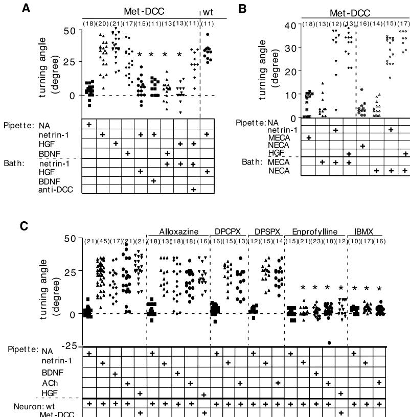
Fig. 4. Test of coreceptor (including adenosine receptor) involvement in netrin responses of Xenopus neurons. (A) Cross-desensitization experiments with DCC and Met ligands. Turning responses of Met-DCC-expressing growth cones induced by a gradient of the indicated ligand in the pipette, in the presence of uniform concentrations of HGF (50 ng/ml), BDNF (50 ng/ml), netrin-1 (100 ng/ml), and/or antibody to DCC (1 \mu g/ml) in various combinations in the bath. Cross desensitization of the HGF response by netrin-1 in the bath can be blocked by antibody to DCC. (Right of the dotted line) In wild-type (wt) neurons, bath-applied HGF does not cross desensitize netrin responses. (B) Cross-desensitization experiments with adenosine receptor agonists on Met-DCC-expressing neurons. The agonists MECA or NECA were delivered from the pipette (1 mM) or applied in the bath (10 \mu M). Similar results were observed with other concentrations in the pipette (100 \mu M and 10 mM of MECA or NECA) or in the bath (100 \mu M of MECA or NECA) (17). (C) Test of adenosine receptor antagonists (present uniformly in the bath) on netrin-induced turning. Alloxazine (10 \mu M), DPCPX (1 \mu M), and DSPSX (1 \mu M) have no effect on turning responses induced by netrin-1 or Ach on wild-type neurons. Alloxazine was also without effect on responses to BDNF or HGF (applied to Met-DCC-expressing neurons). DPCPX and DSPSX at 10 \mu M were also without effect on netrin and Ach-induced turning, and alloxazine at 30 \mu M was without effect on netrin-induced turning (17). Enprofylline (10 \mu M) and IBMX (10 \mu M) abolished the turning responses to all the ligands tested, which are indicated in the chart (HGF effects were tested on Met-DCC-expressing neurons). *, statistically significant change compared with no-drug condition ( P < 0.001 , Student's t test).
